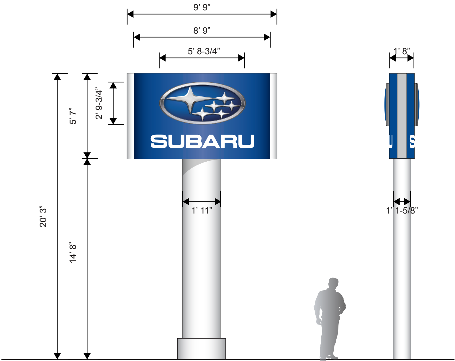
E01 - P50 2019 PYLON Scale: 1/4" = 1' 0"
