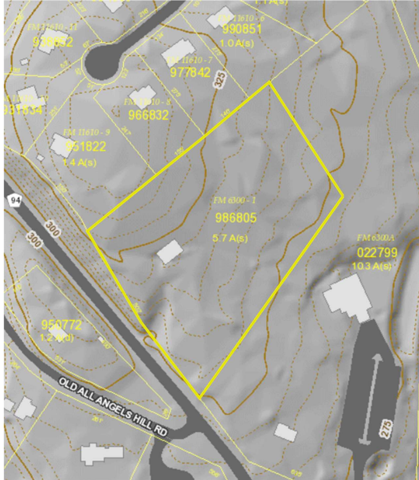
Figure C – USGC Map
