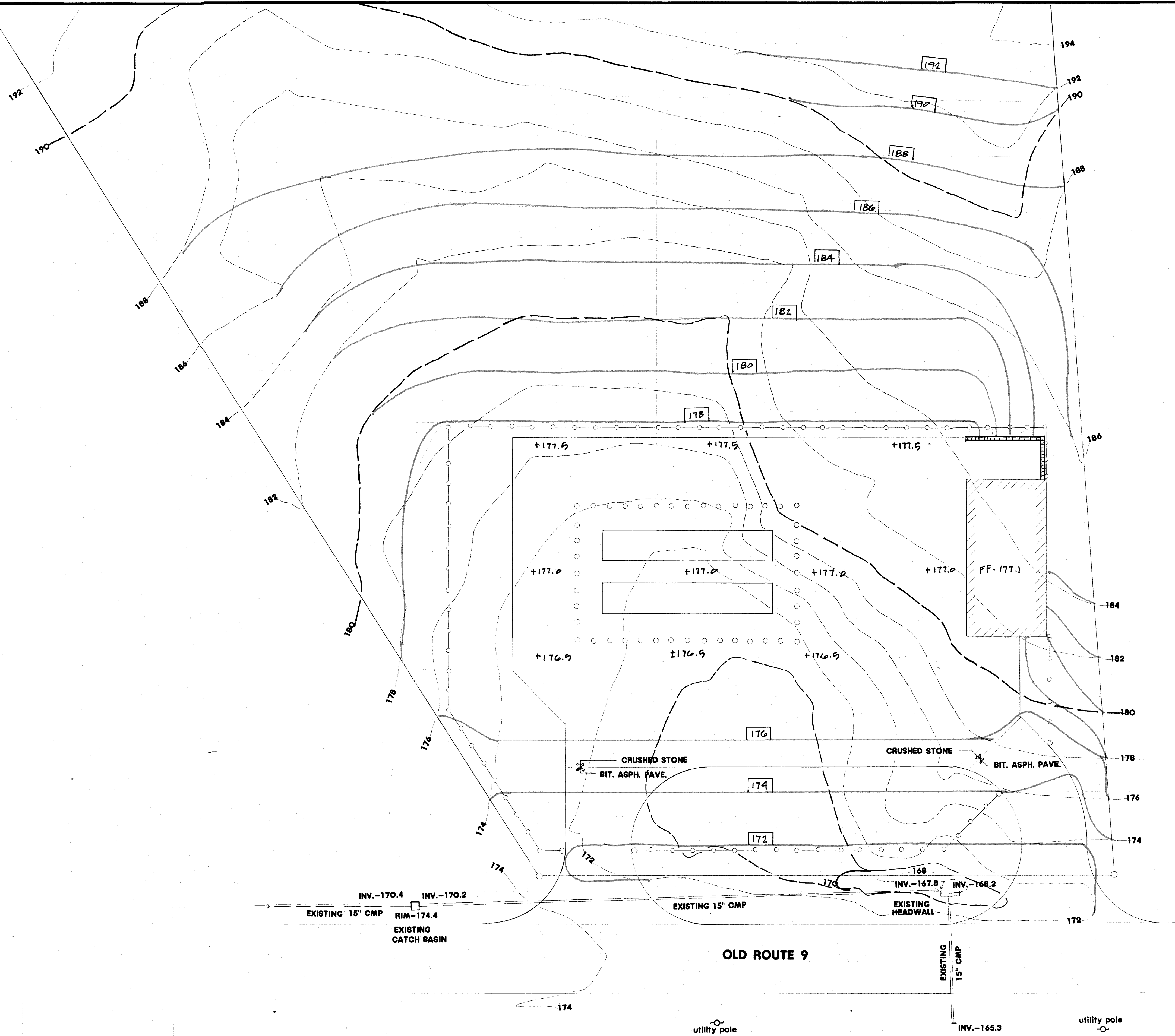
GRADING & DRAINAGE PLAN (CONCEPTUAL)
